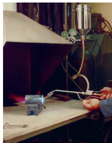
Detached production hopper permits continuous spraying
